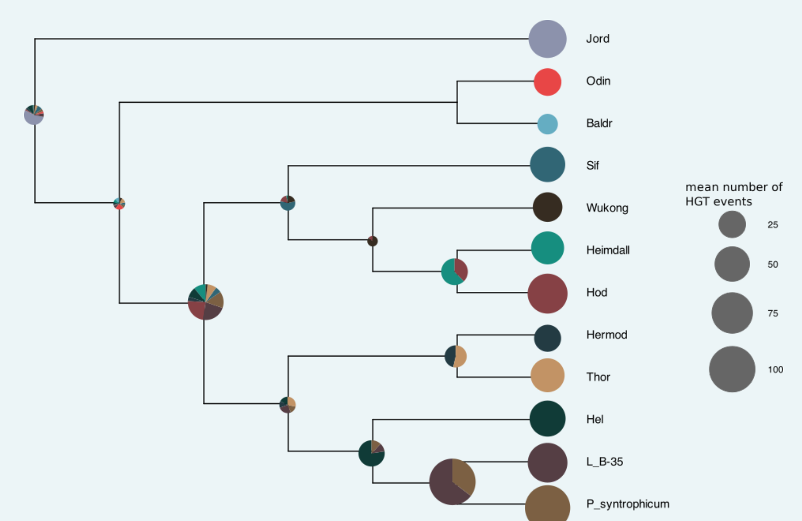
Figure 5: Acceptor analysis. The acceptor was defined as the MRCA of the biggest Asgard monophyletic group stemming from the seed protein. Eukaryotic sequences were considered de facto Heimdall. Sub-lineage transfers are collapsed to the tip node.
