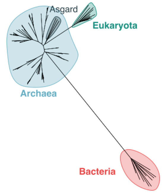
Figure 1: Tree of Life. Adapted from Williams et al. (2020)
