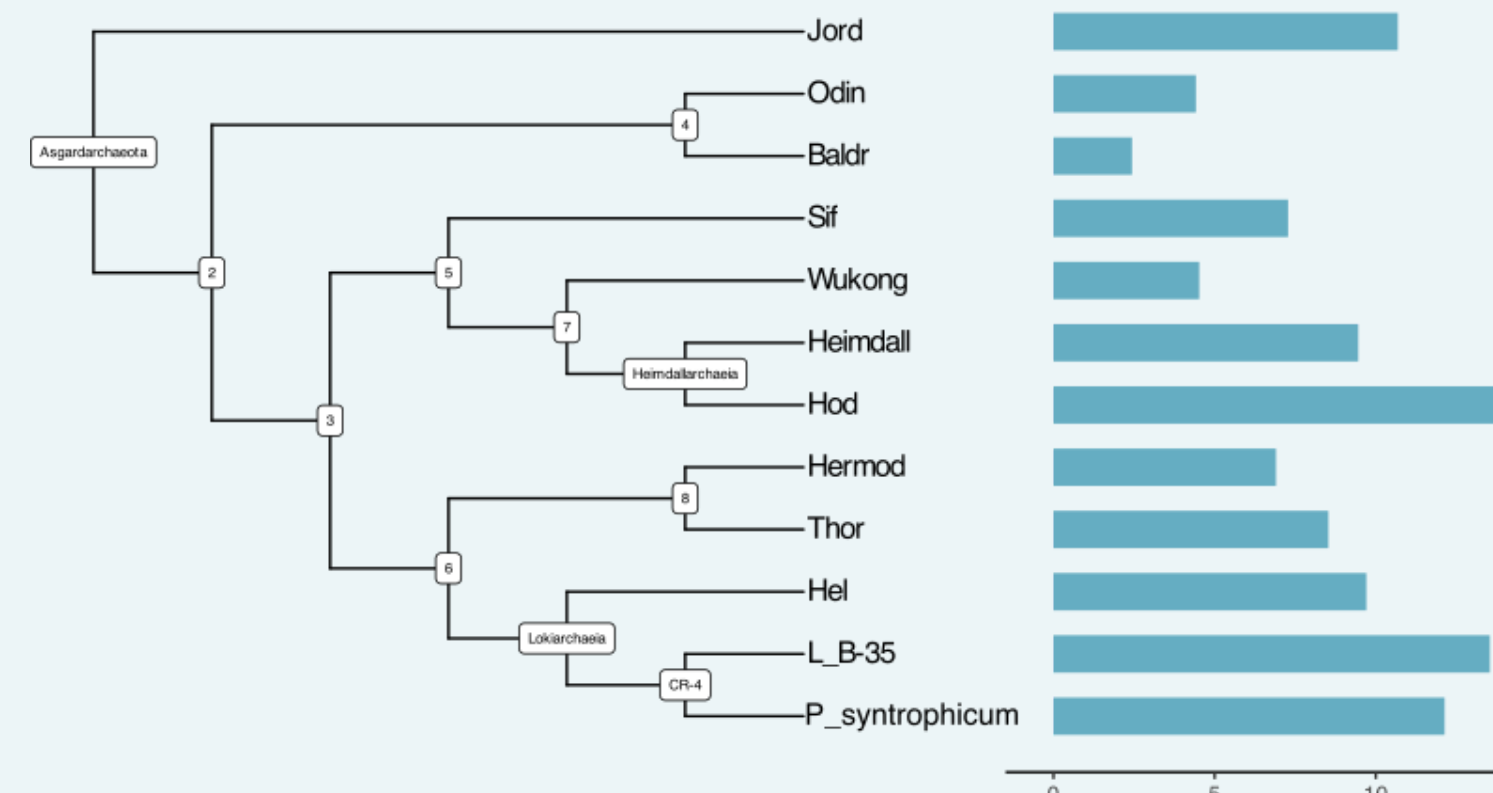
Figure 4: Percentage of transferred genes relative to the whole proteome. Proteins were considered HGTs if the sister group contained less than 10% sequences of archaeal origin, and was assigned the donor taxa as the MRCA of at least 50% leaves.
